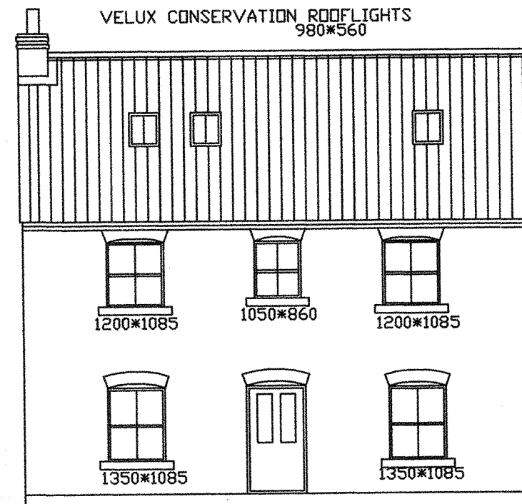
FRONT ELEVATION (NORTH)
