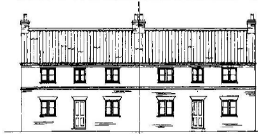
SOUTH FRONT ELEVATION
